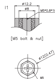
A Detail Drawing
